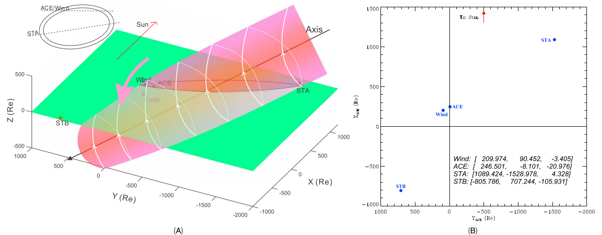
Figure 7. (a) The spatial morphology of the SFR. The details are presented in the text. (b) The spacecraft positions in the ecliptic plane (GSE coordinates in Earth radii ( R_E )). The blue dots indicate the spacecraft positions with their names following, and the right bottom presents their detailed positions in units of R_E .
